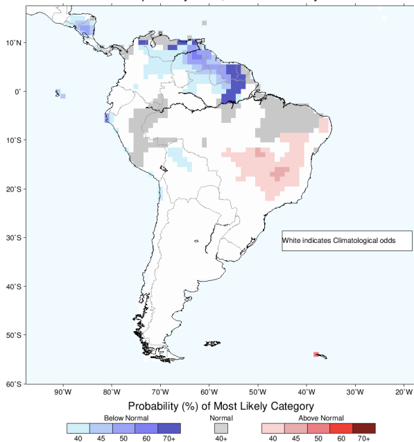
IRI Multi-Model Probability Forecast for Temperature for March–April–May 2021, Issued February 2021
